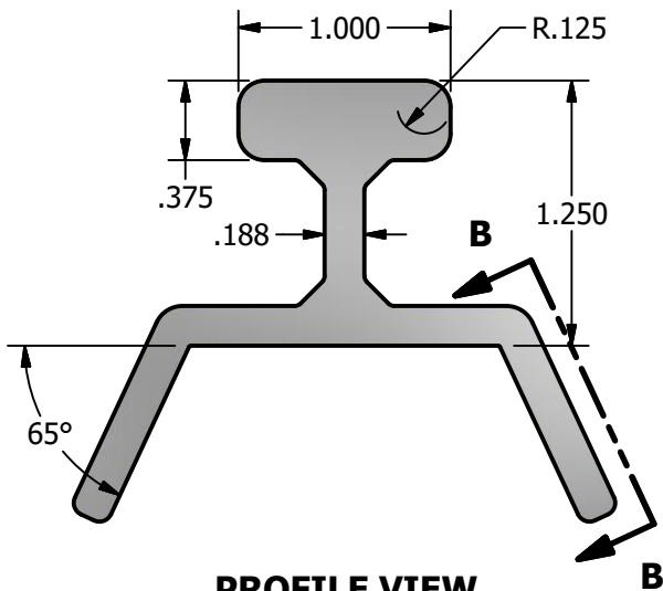
PROFILE VIEW
