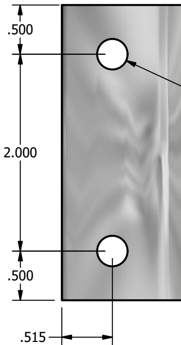
SECTION B-B
