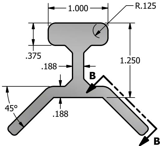
PROFILE VIEW
